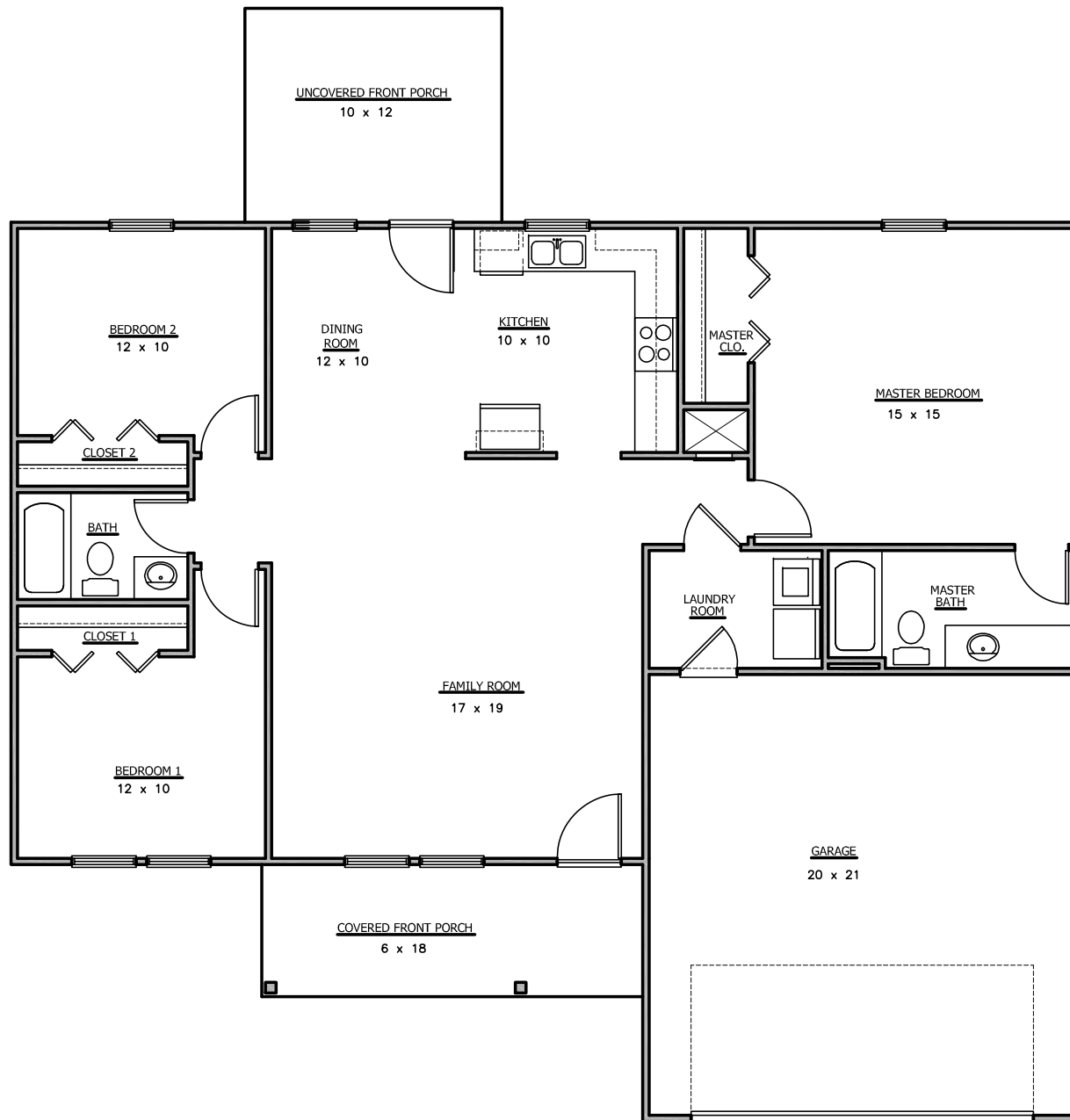
EDGEWOOD FLOOR PLAN
