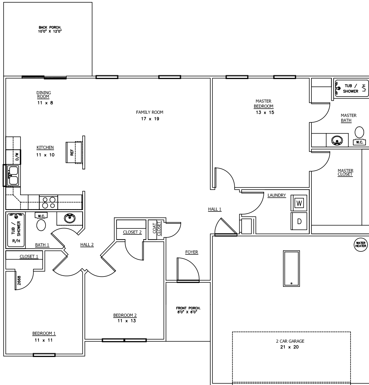
SULLIVAN - 1ST FLOOR PLAN
